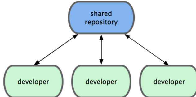
Figure 5.1: Centralized workflow
