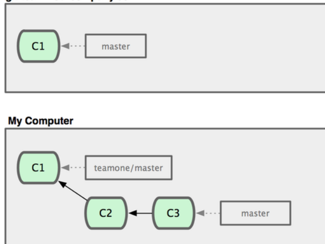
Figure 3.36: Clone a repository, and base some work on it.
